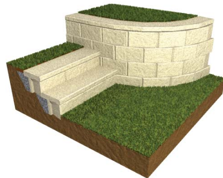
- Capping -
