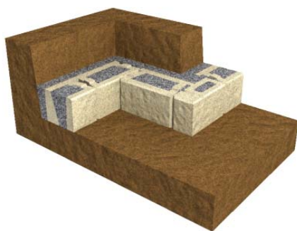
- First Course -
